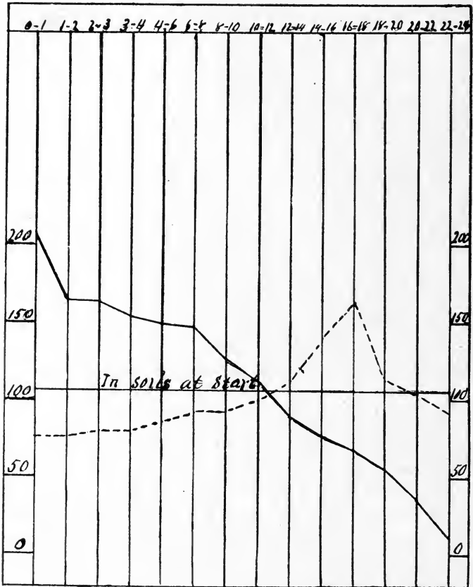
FIG. 5.—Showing distribution of water-soluble sulphates after capillary movement. Solid line indicates results after 50 days; broken line, results after 20 days. Values are means for 8 soil types.
